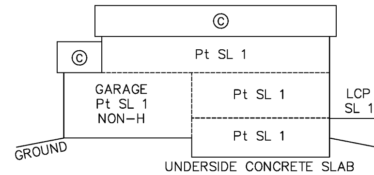
SECTION B-B'
