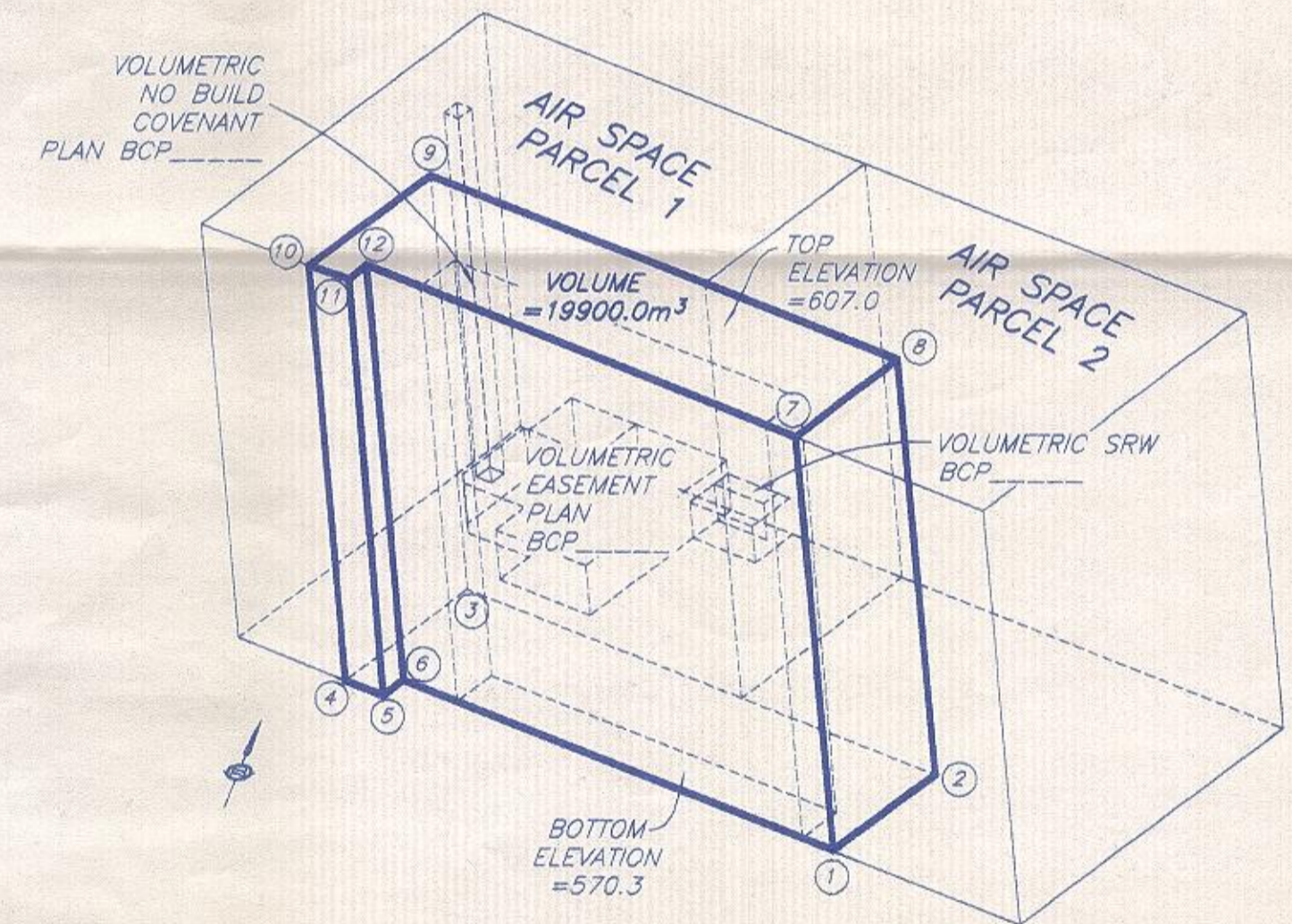
ISOMETRIC VIEW NOT TO SCALE
