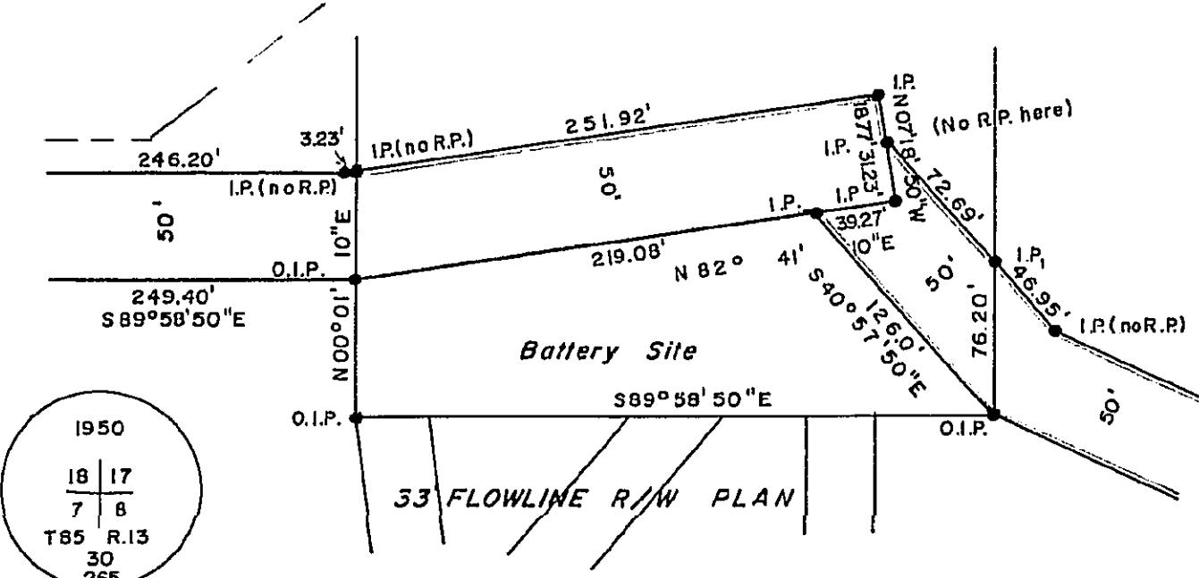
DETAIL A: 1" = 100'
